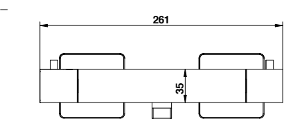
Cod. 43543CRPR Miscelatore termostatico doccia esterno Thermostatic external shower mixer
