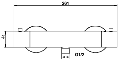
Cod. 32553CRPR Miscelatore termostatico doccia esterno Thermostatic external shower mixer
