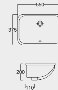
A 118 NETTUNO LAVABO SOTTOPIANO 55x37,5x20 NETTUNO UNDER COUNTER WASHBASIN 55x37,5x20
