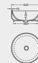
G42 LAVABO APPOGGIO TONDO 42 COUNTERTOP ROUND WASHBASIN 42
