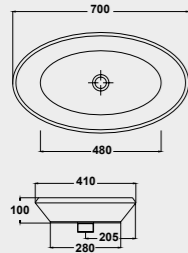
AC53 LAVABO D'APPOGGIO OVAL 70x41x10 OVAL COUNTERTOP WASHBASIN 70x41x10
