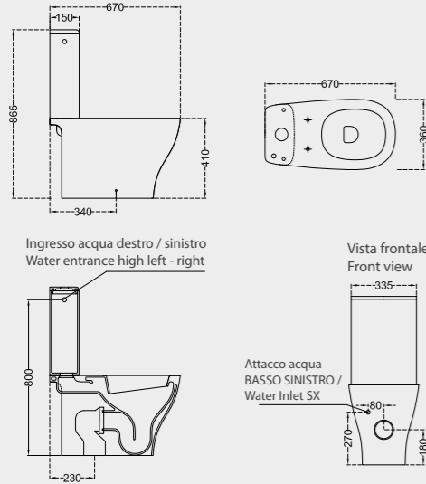
M12 WC MONOBLOCCO + M18 CASSETTA CERAMICA CLOSE-COUPLED WC + CERAMIC CISTERN
