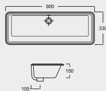
A 110 GEA LAVABO SOTTOPIANO 90x33x15 GEA UNDER COUNTER WASHBASIN 90x33x15
